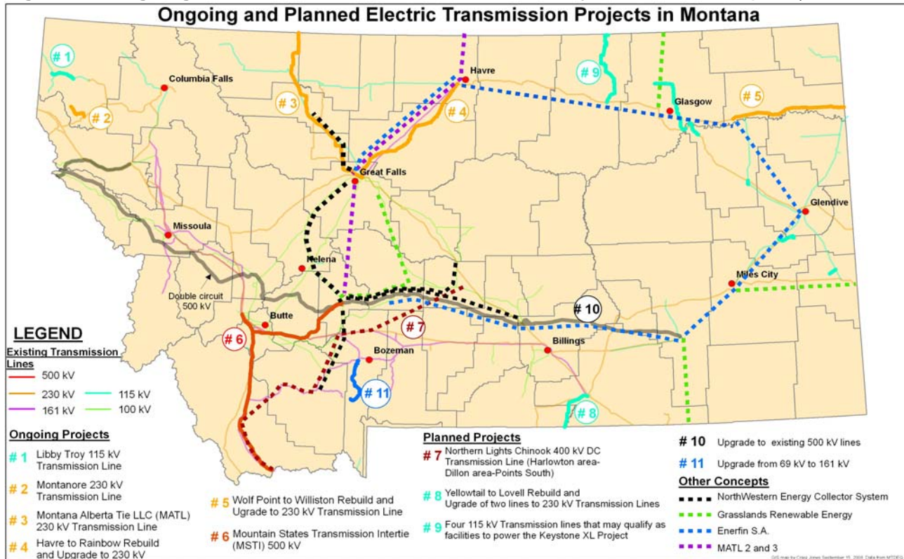
Figure T5. Ongoing and Planned Electric Transmission Projects in Montana (DEQ)
