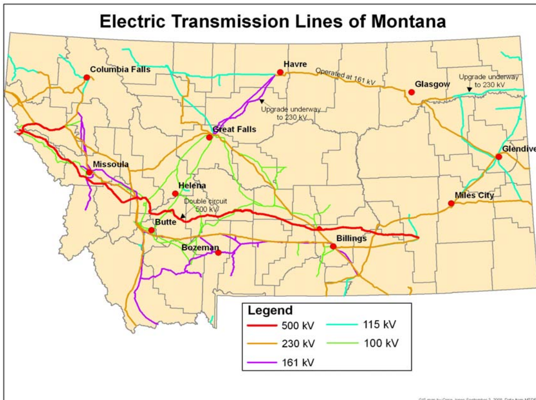
Figure T1. Electric Transmission Lines of Montana as of 2009 (Montana DEQ)
