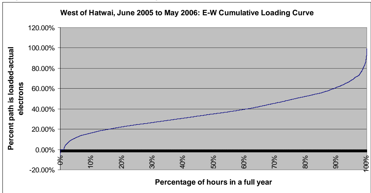
Figure T3. West of Hatwai path cumulative loading curve June 2005-May 2006 (Negative flows mean power was flowing from west to east)
